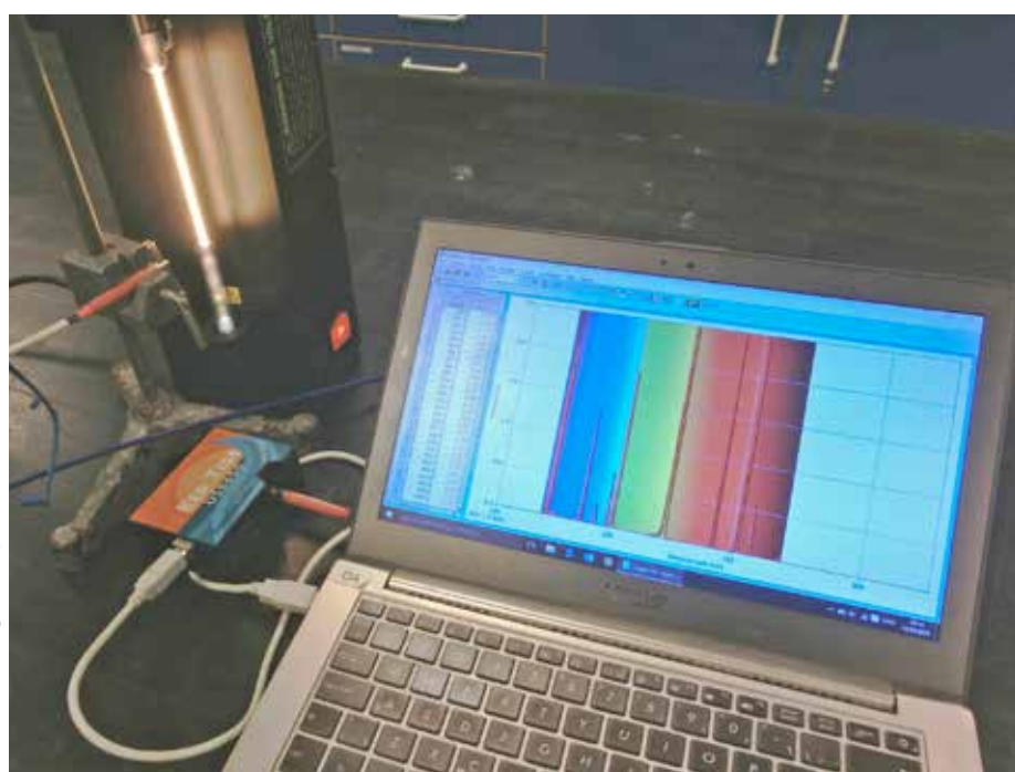
Record of the mercury spectrum with the Ocean Optics Red Tide spectrometer and the programme LoggerPro.
